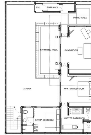
GROUND FLOOR PLAN WINGS SCALE 1:100
