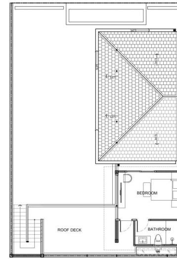
SECOND FLOOR PLAN WINGS SCALE 1:100 HALL 33 03/02/2012
